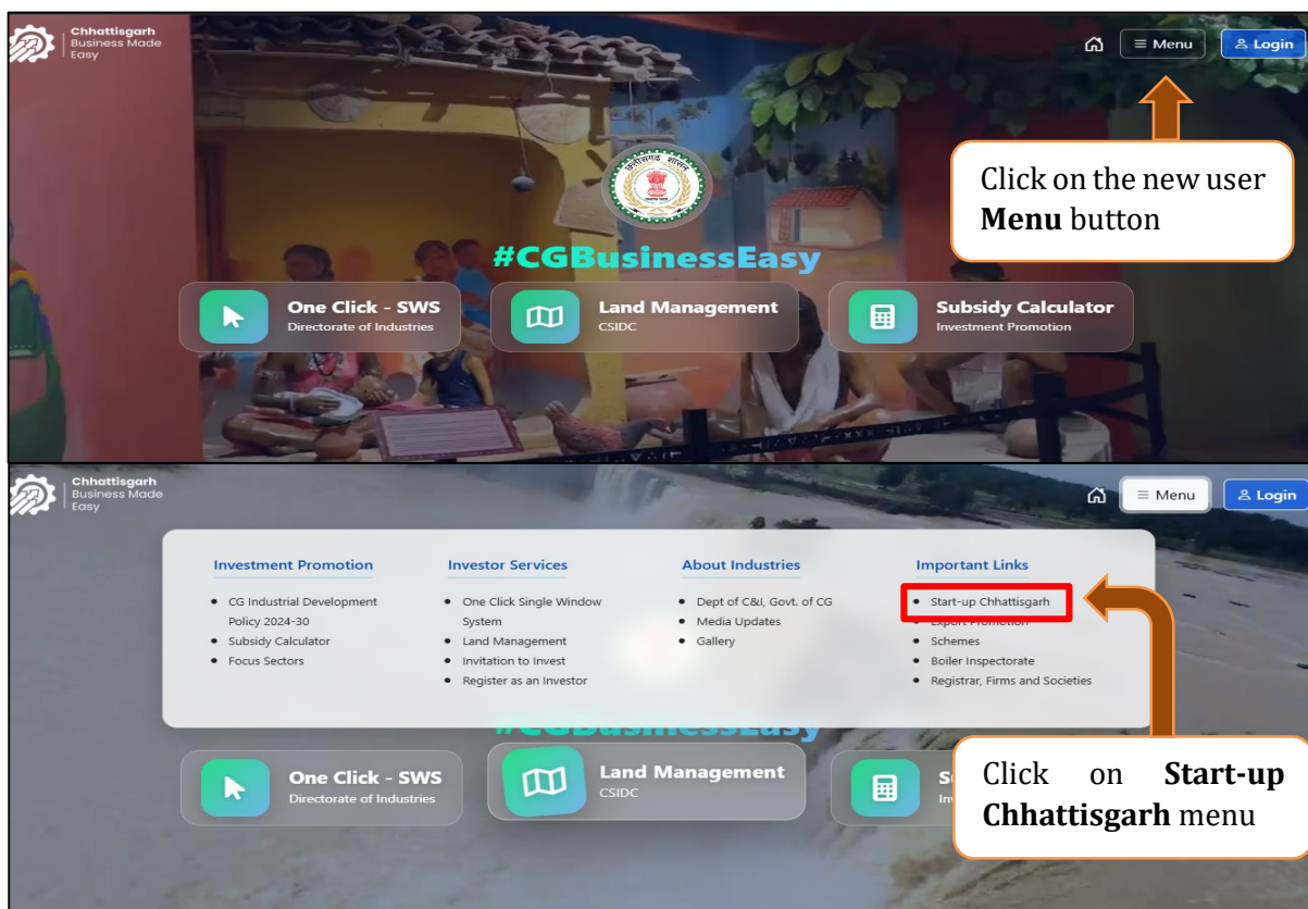
Figure 3.1: Homepage Screen
